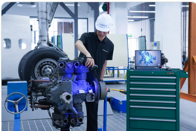
An aircraft piston engine scanned on its stand. The mesh builds on the laptop in real time.
